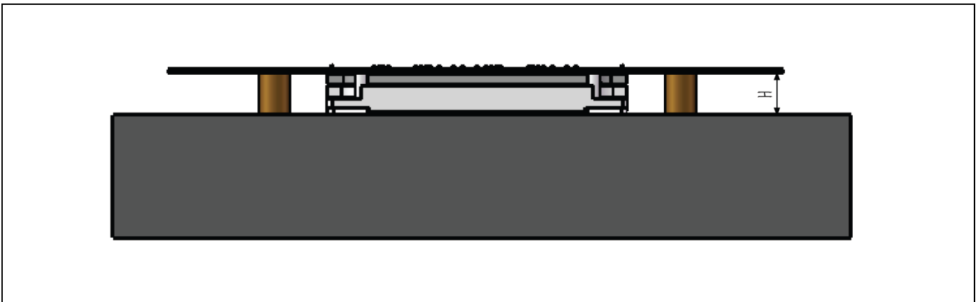
Figure 2: Mounting a PCB to the heat sink.
