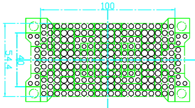
Figure 4: The areas of the C6S base plates where TIM is applied.
