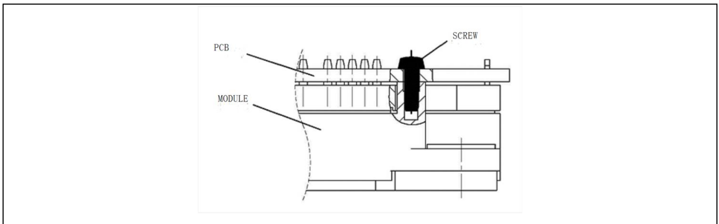
Figure 6: Align PCB to the power module.
