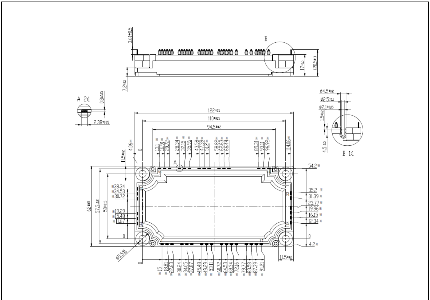
Figure 1: Technical drawing of C6-module.
